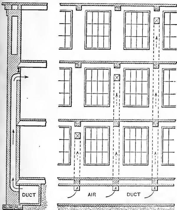
FIG. 6. ANOTHER FLUE ARRANGEMENT ADAPTED TO STANDARD MILL CONSTRUCTION
